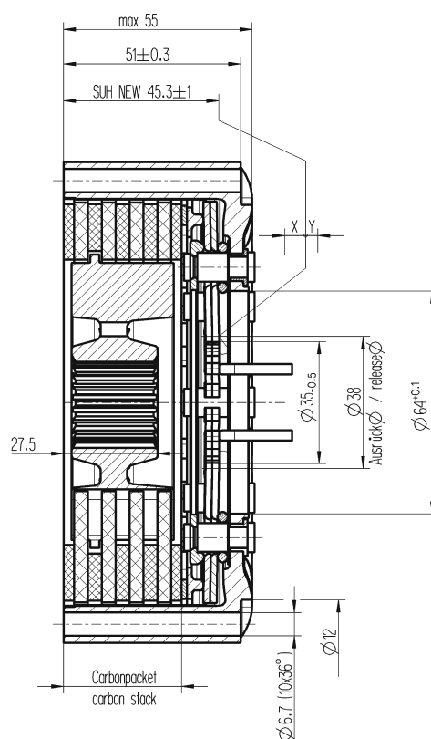
4-Scheiben-Kupplung 4-disc clutch (Formula 4/115 Carbon)
