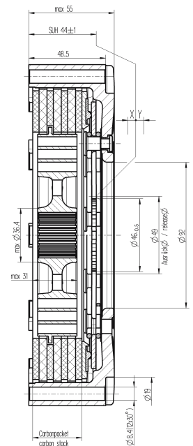
3-Scheiben-Kupplung 3-disc clutch (Formula 3/184 Carbon)
