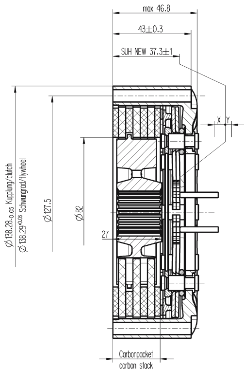
3-Scheiben-Kupplung 3-disc clutch (Formula 3/115 Carbon)
