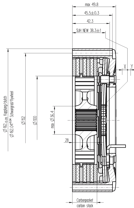
3-Scheiben-Kupplung 3-disc clutch (Formula 3/140 Carbon)
