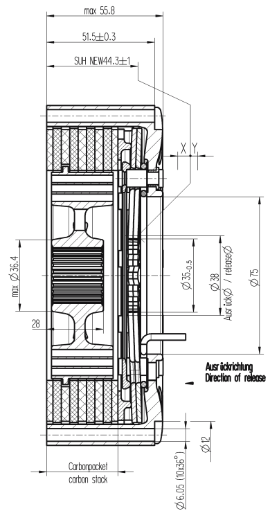
4-Scheiben-Kupplung 4-disc clutch (Formula 4/140 Carbon)
