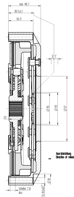
1-Scheiben-Kupplung 1-disc clutch (RCS 1/200 Sinter-Pad torsion)
